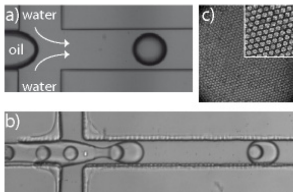
Figure 1: a- Droplet formation at a cross junction. b- Complex droplet formation at a cross junction (double emulsion). c- Crystal of droplets.
