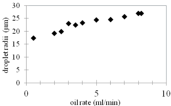
Figure 4: Measured droplet radii obtained by detection when oil rate is varying. The water rate is constant (5 \mu l/min and 80 \mu l/min).
