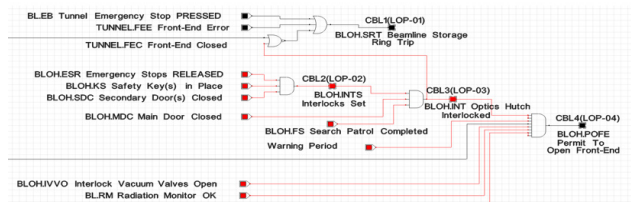
Figure 3: Extract of the logic for one beamline. Permit to open the front-end.
